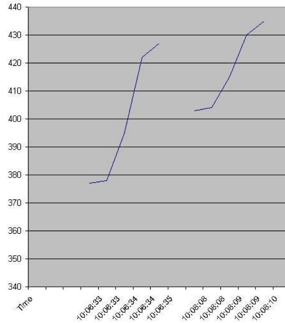
Figure 7. Billet temperature measurements
